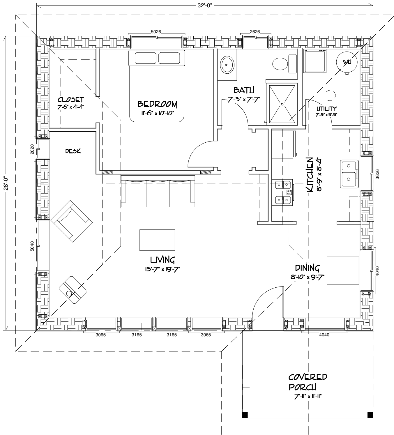
FLOORPLAN 896 SQ.FT.
