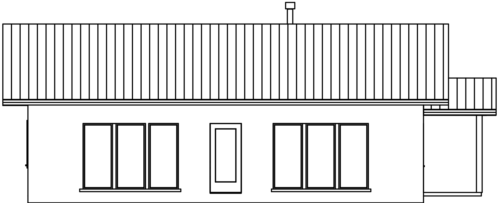
SOUTH ELEVATION
