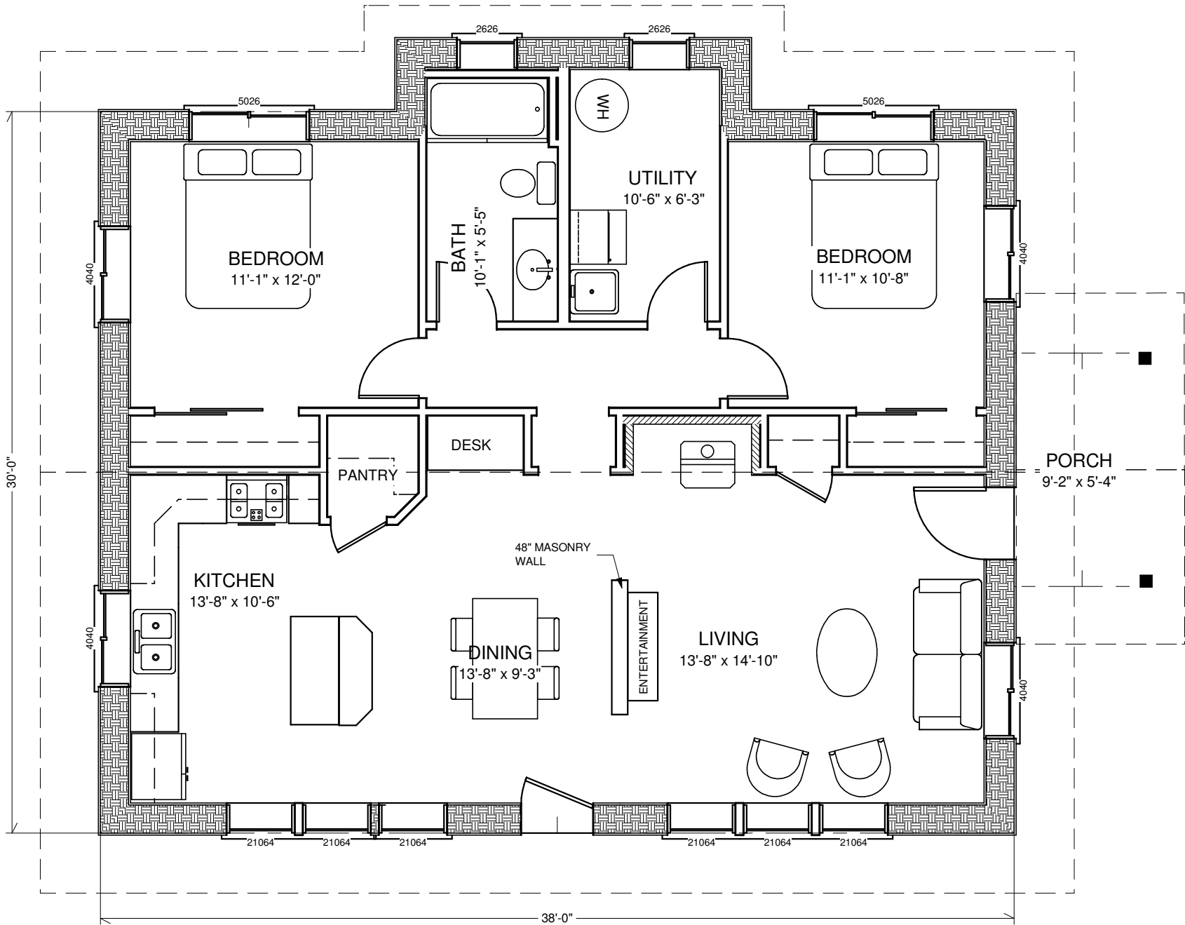
FLOORPLAN 1180 SQ.FT.
