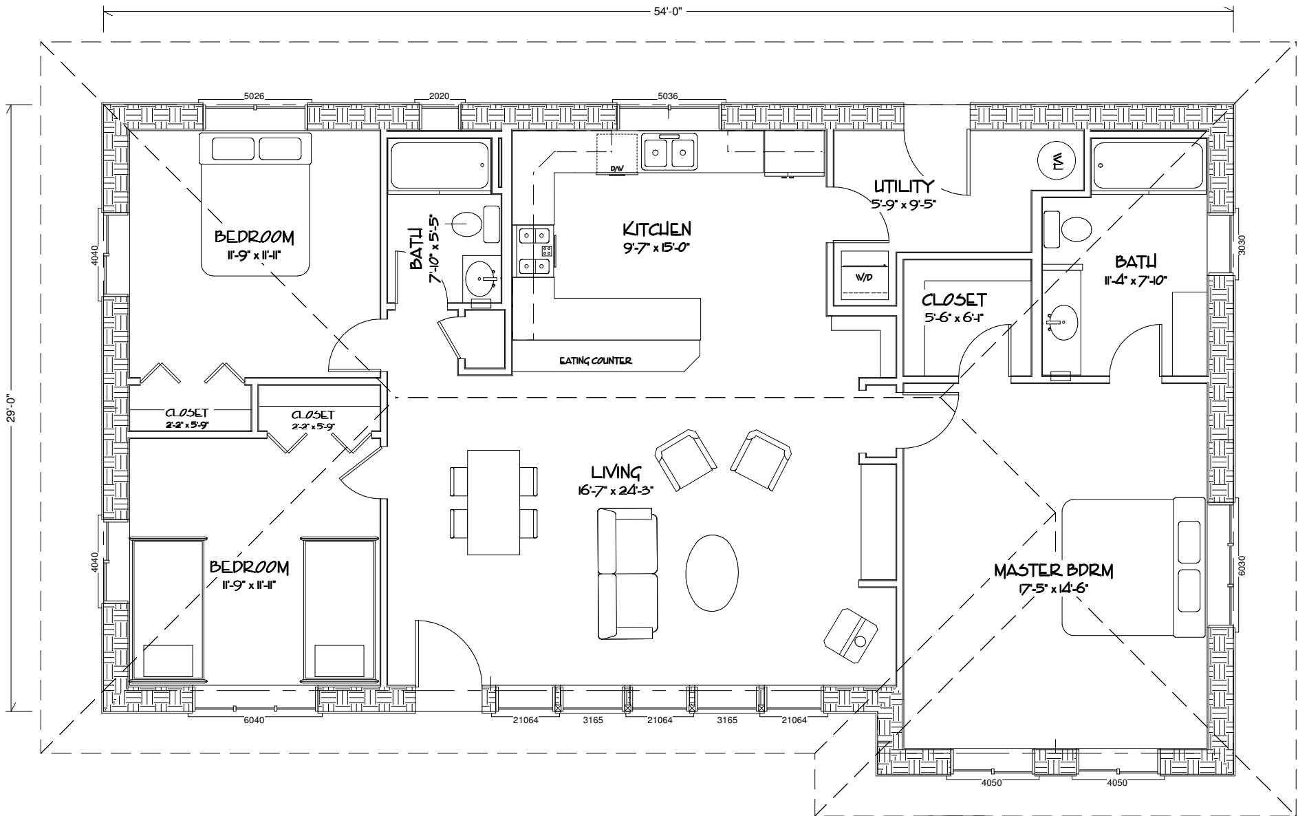
FLOORPLAN 167 SQ.FT
