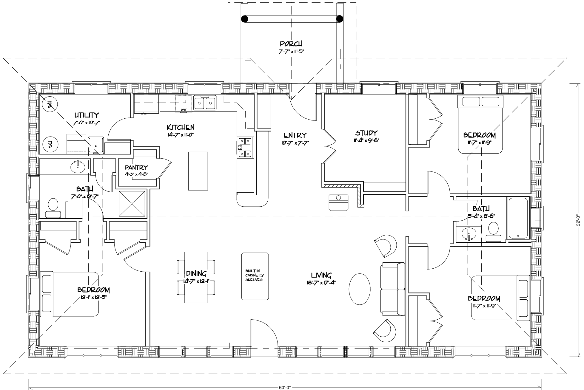
FLOORPLAN 1920 SQ.FT.
