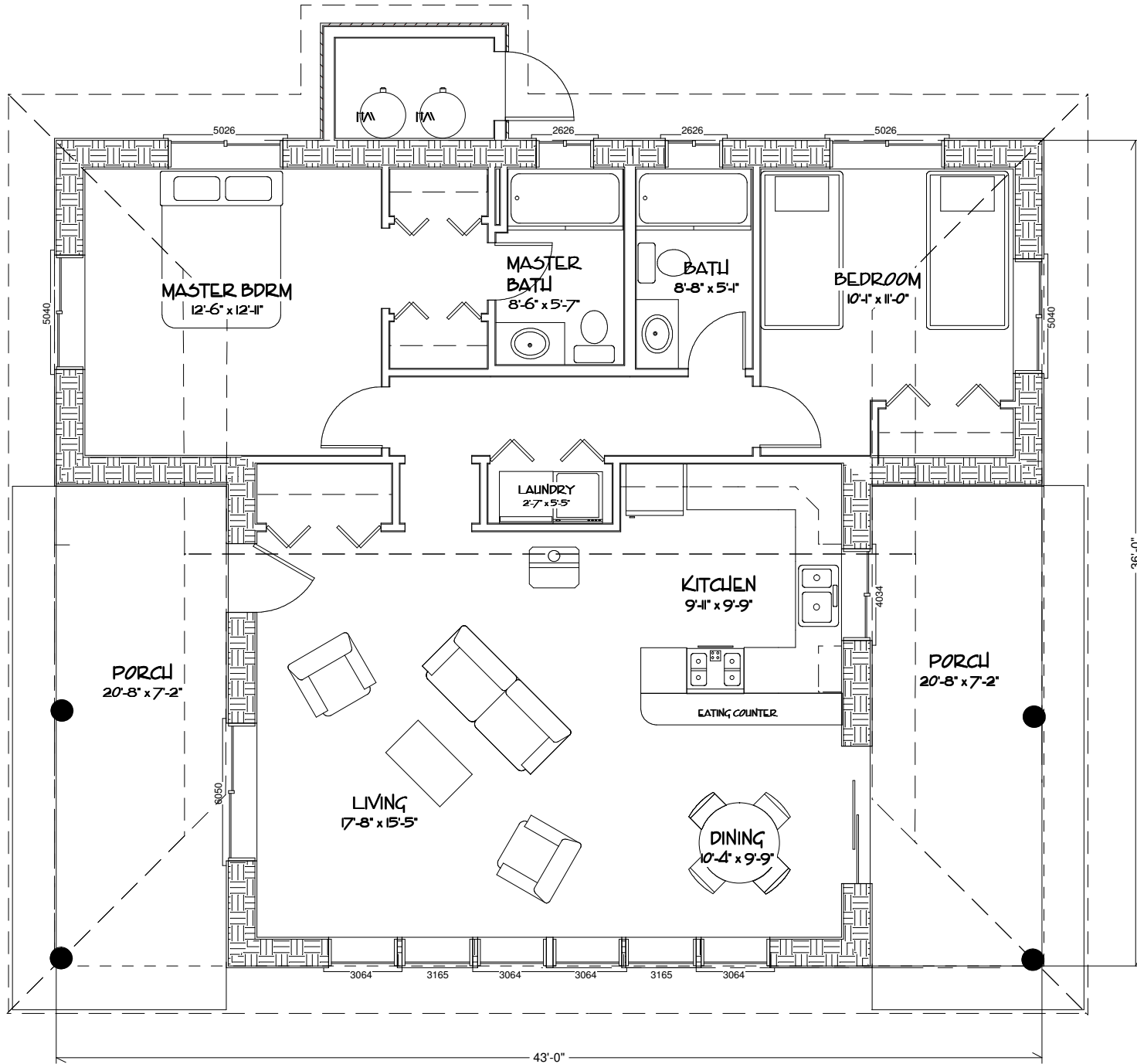
FLOORPLAN 1233 SQ.FT.
