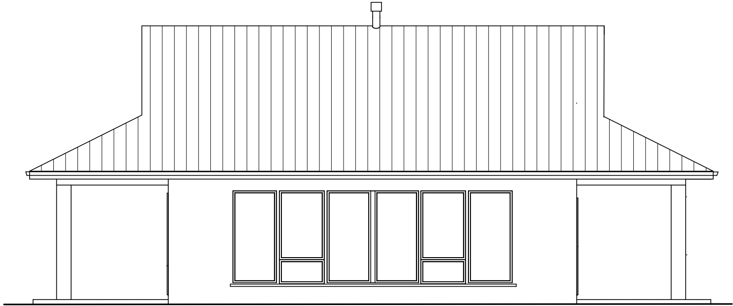
SOUTH ELEVATION
