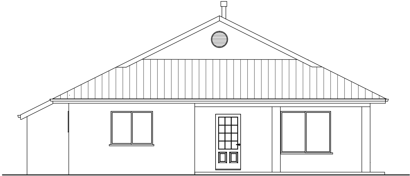
WEST ELEVATION
